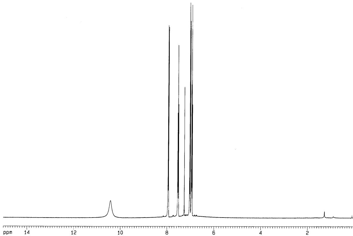
Figure 1. Compound X's ^1\text{H} NMR spectrum.
