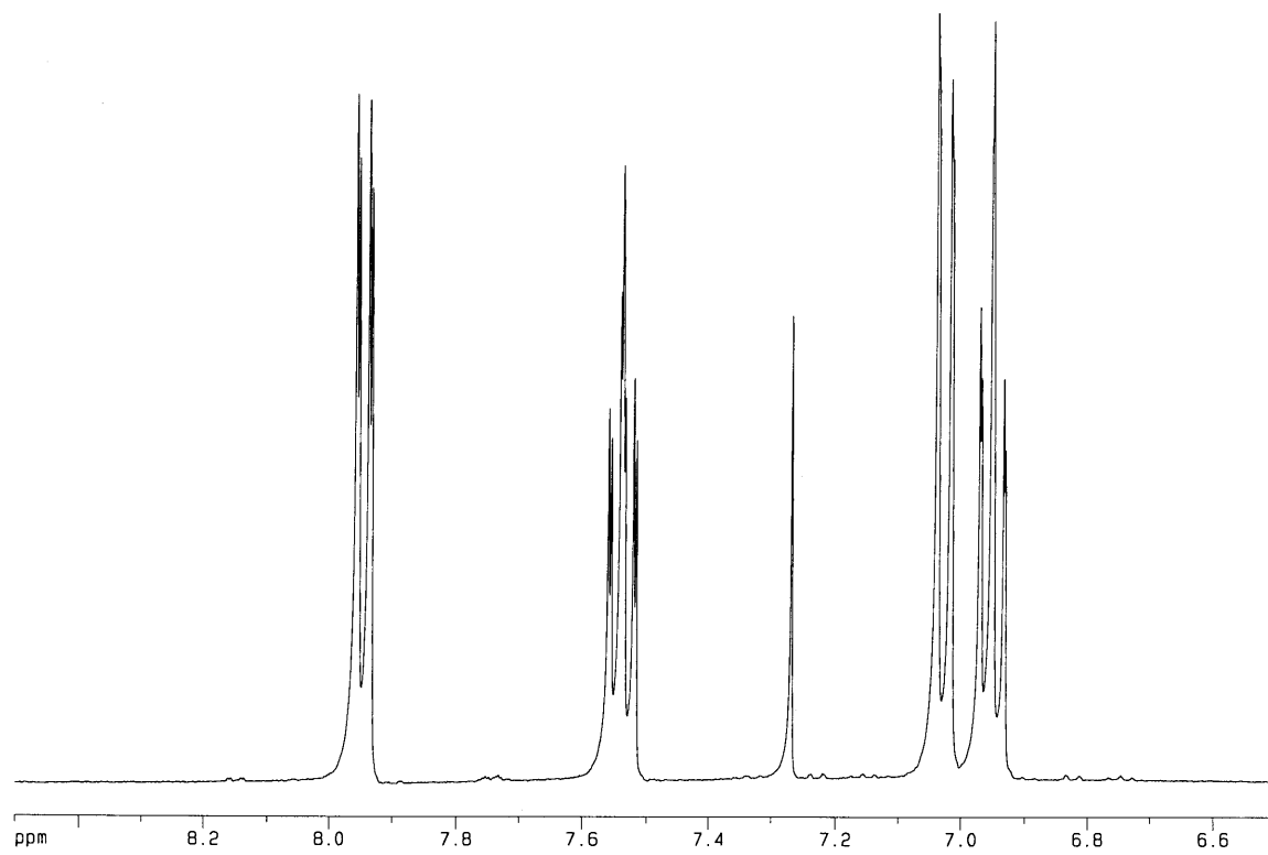
Figure 2. Expanded ^1\text{H} NMR spectrum of Compound X.
