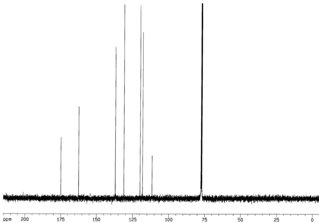
Figure 3. Compound X's ^{13}\text{C} NMR spectrum.
